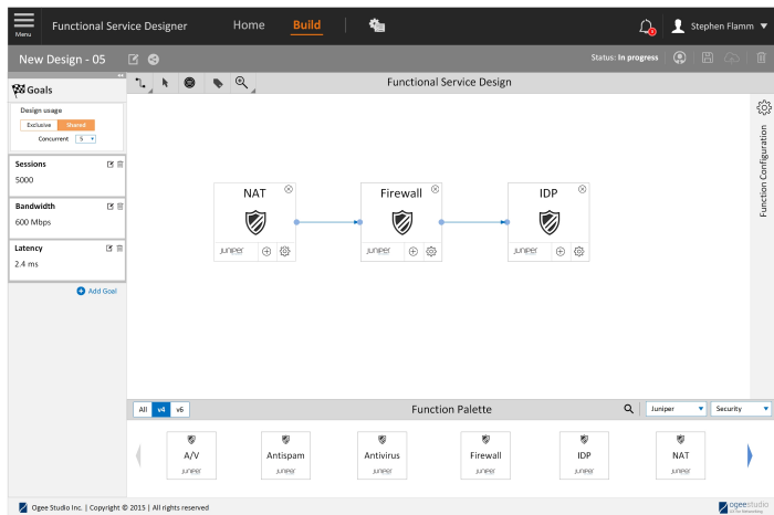
Network Function Designer
